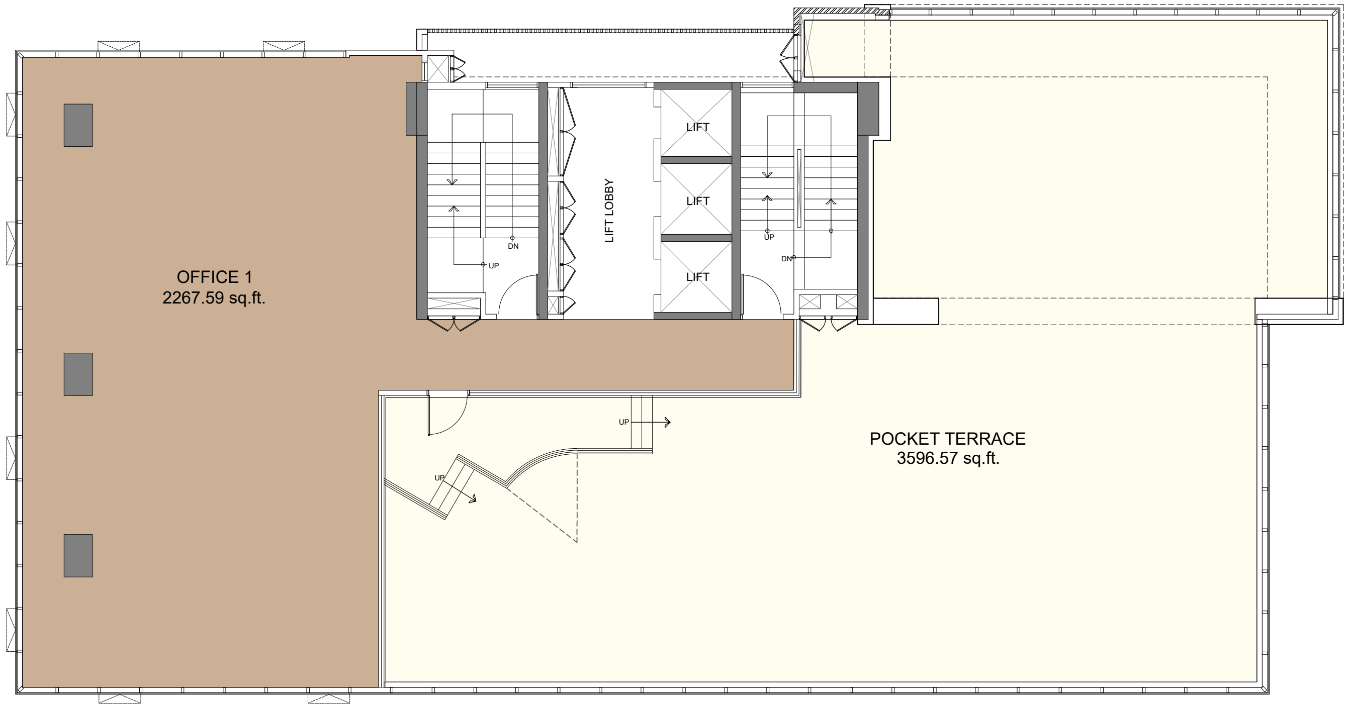
NINTH FLOOR PLAN USABLE AREA = 2267.59 SQ.FT.
